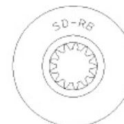
For DF 60, DF 70 DT 75 - 140 Thrust Washer 13 Tooth Spline
